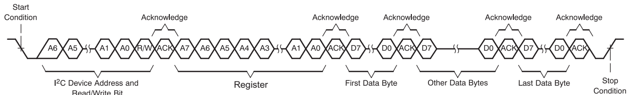
Figure 45. Multiple-Byte Write Transfer
