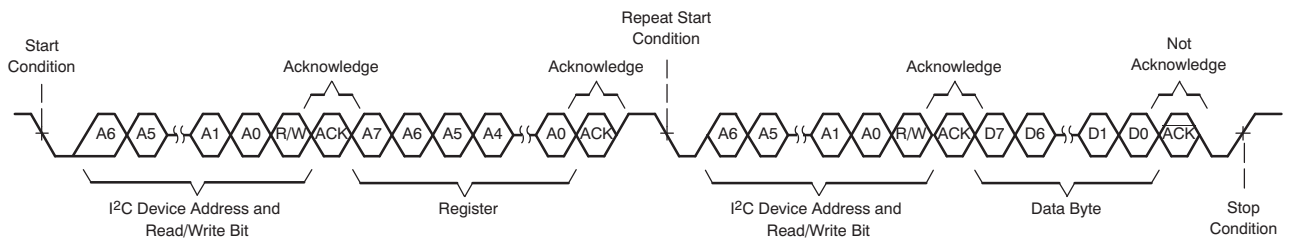
Figure 46. Single-Byte Read Transfer
