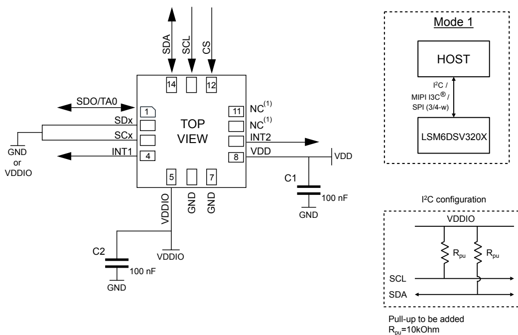
Figure 27. LSM6DSV320X electrical connections in mode 1
