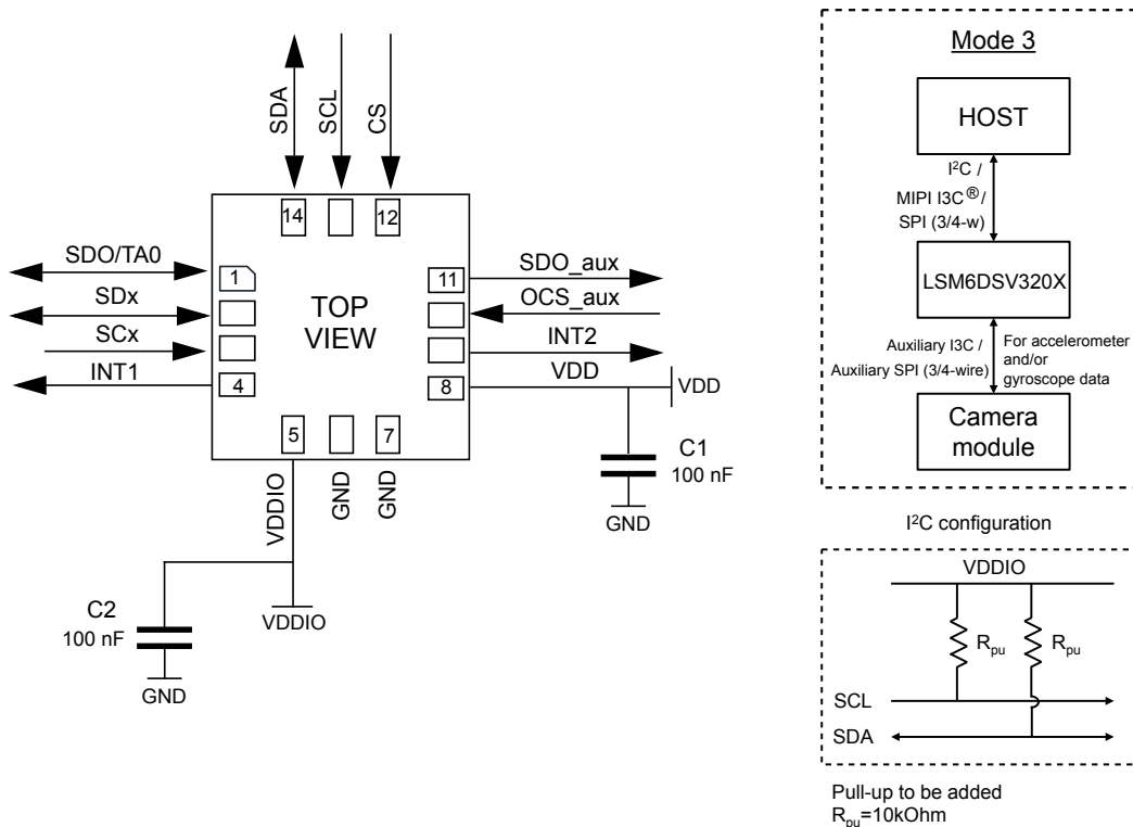
Figure 29. LSM6DSV320X electrical connections in mode 3 (auxiliary 3/4-wire SPI or auxiliary MIPI I3C)
