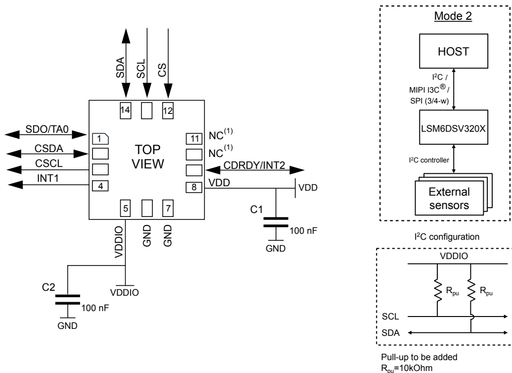
Figure 28. LSM6DSV320X electrical connections in mode 2
