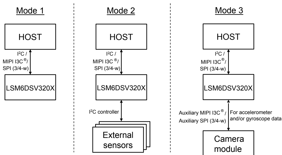
Figure 6. LSM6DSV320X connection modes
