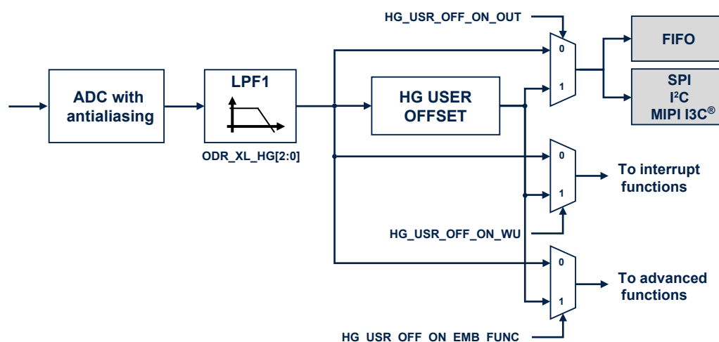
Figure 20. High-g accelerometer filtering chain
