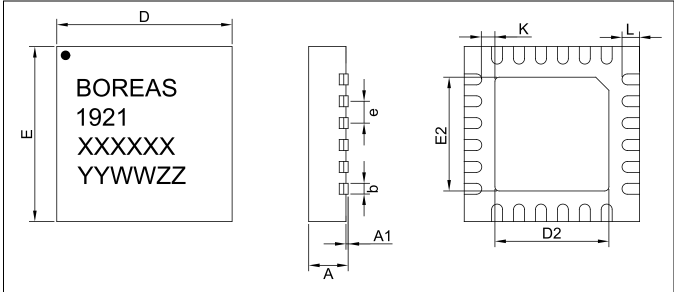
Figure 41: QFN 24L 4.0mm × 4.0mm package outline drawing
