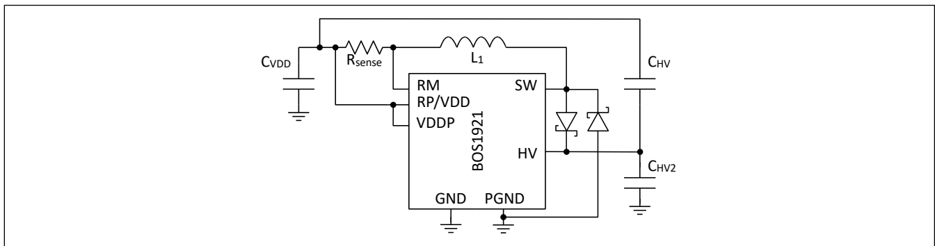
Figure 39: Simplified schematic with a Schottky diode between SW/HV and SW/PGND pins for noise reduction
