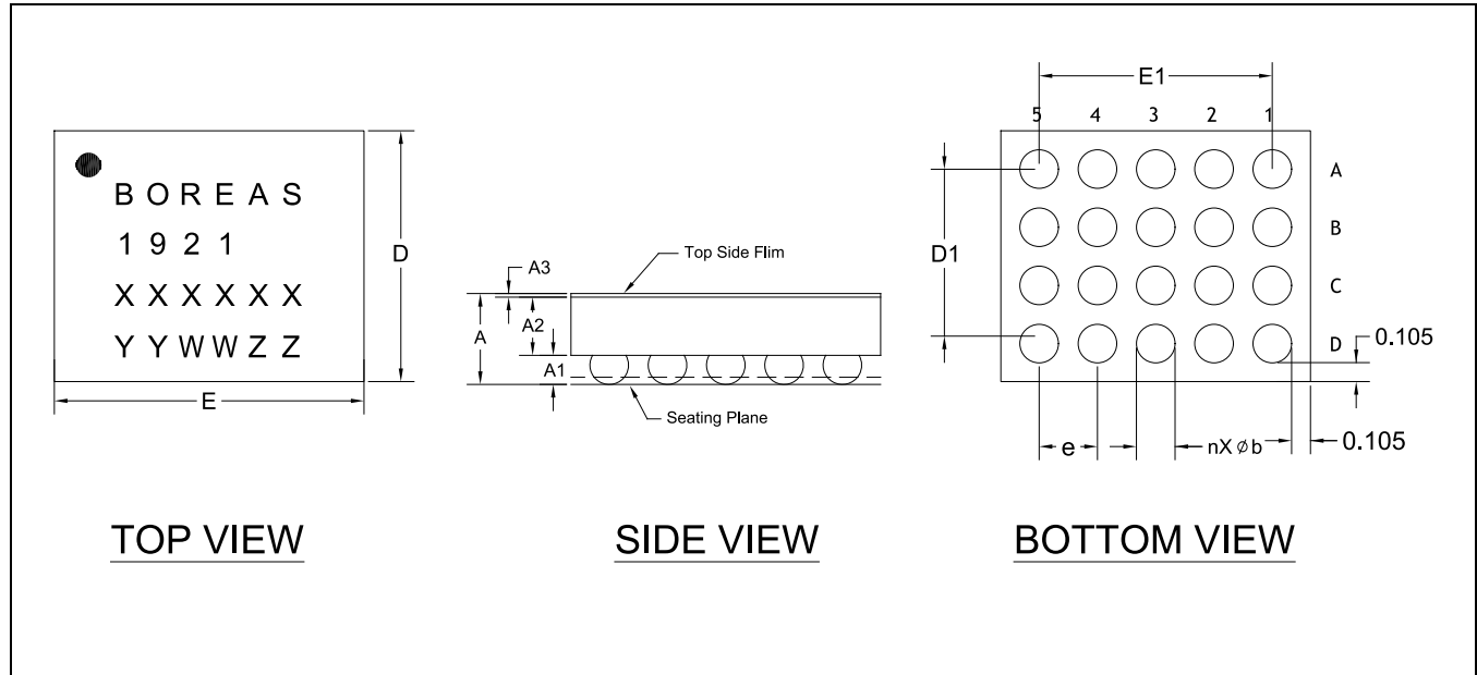
Figure 43: WLCSP 20B 2.1mm x 1.7mm package outline drawing with top, side, and bottom view
