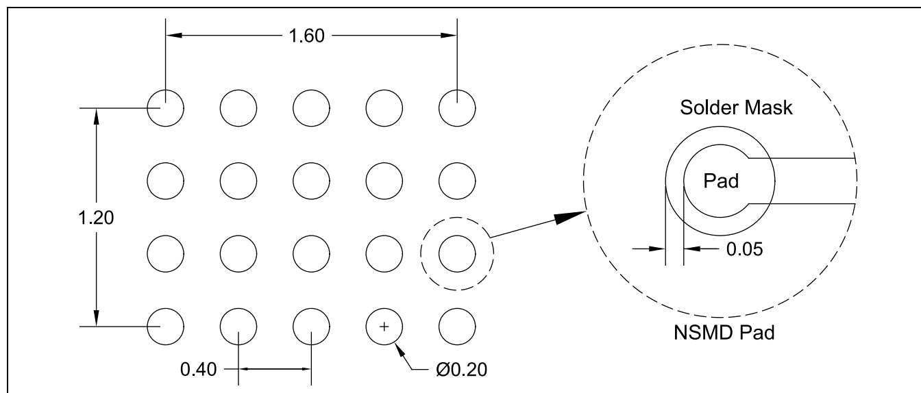
Figure 44: WLCSP 20B 2.1mm × 1.7mm soldering footprint (NOT TO SCALE)
