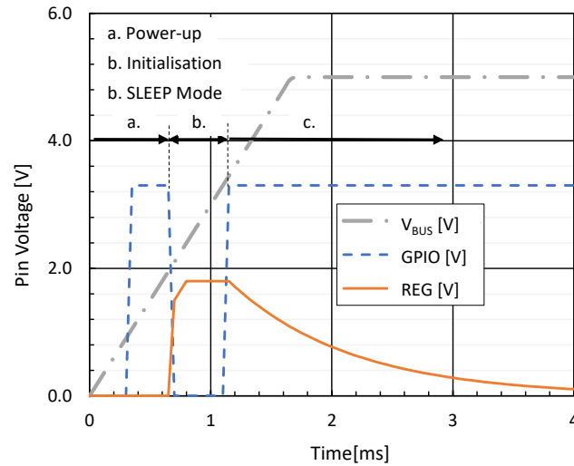
Figure 38: Typical V_{BUS} , GPIO & REG pin voltage during initialisation
