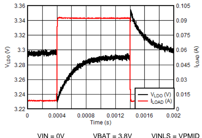
Figure 99. LDO Load Transient - VLDO = 3.3V
