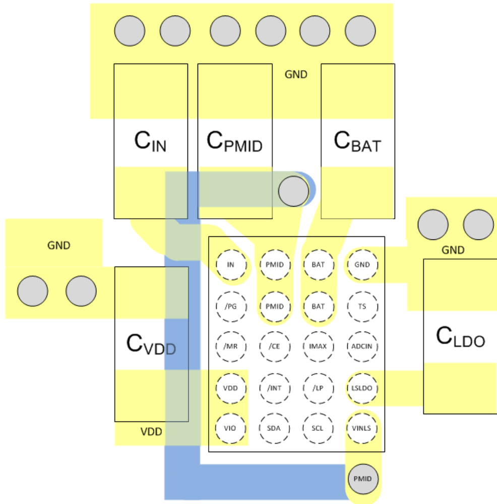
Figure 101. Layout Example
